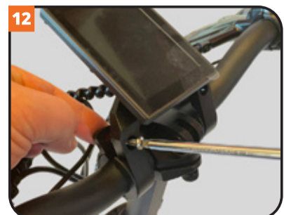
12 Refit the clamp mounting screws – do not overtighten
