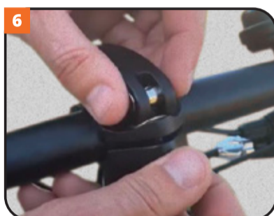
Tighten the bolt into the clamp making sure to leave some slack for later adjustment
